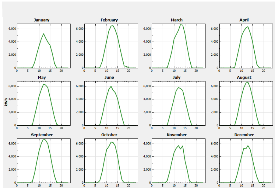
Figure 5.6 (a): Monthly Solar Energy Variation of Hambantota 10MW Plant
