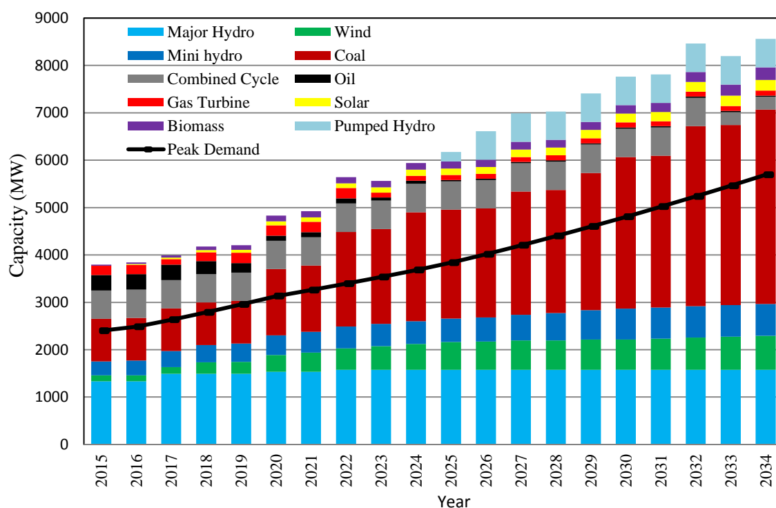
Figure 7.1 –Cumulative Capacity by Plant Type in Base Case
