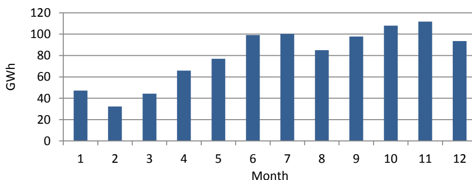
Figure 5.4: Average Monthly Energy Output of Existing Mini hydro Capacity 293.3MW
