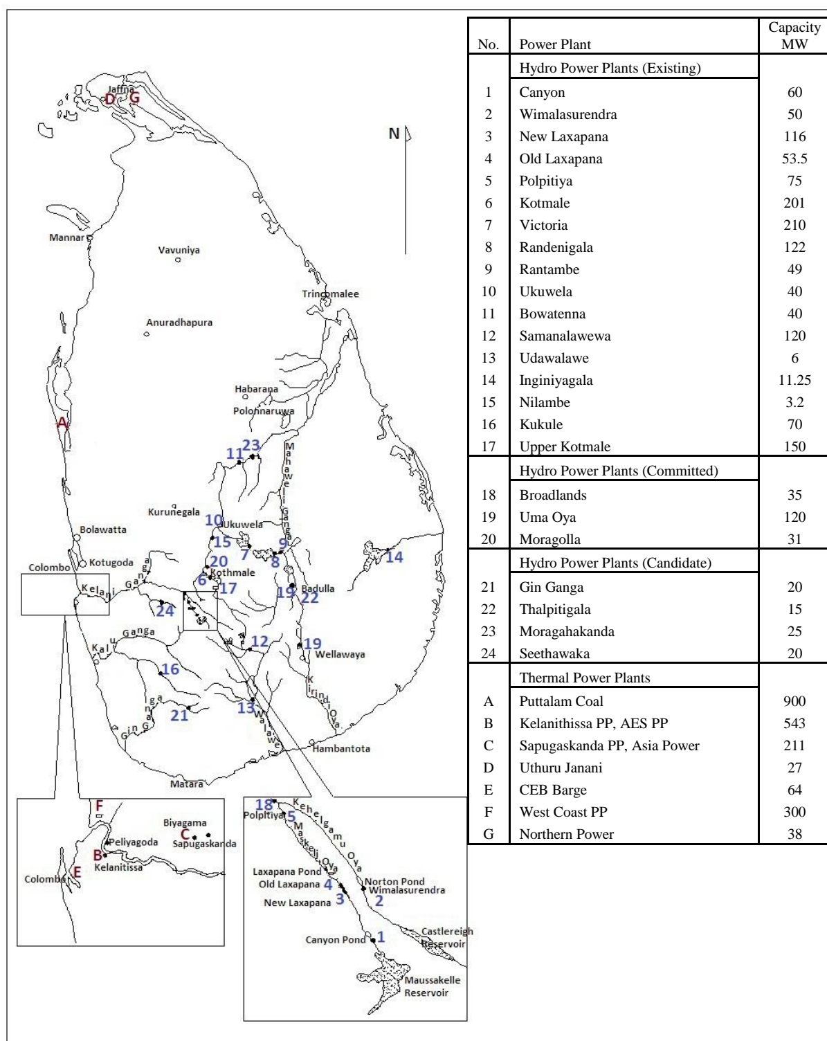
Figure 2.1 - Location of Existing, Committed and Candidate Power Stations
