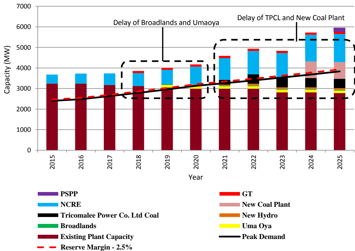
Figure 8.4 - Base Case Plan Cumulative Capacity Addition with Plant Delays
